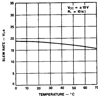
Slew Rate vs Temperature (μA715C)
