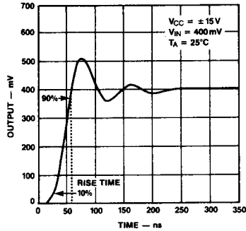
Voltage Follower (Note 1)
