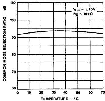
Common Mode Rejection Ratio vs Temperature (μA715C)
