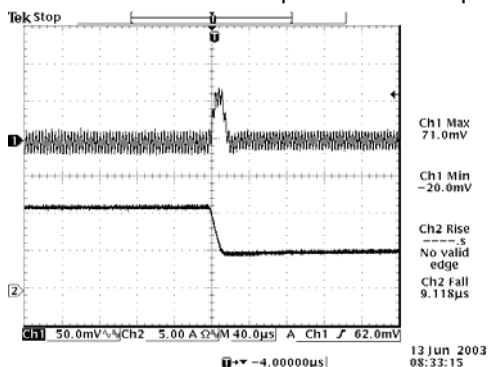
100% to 50% load 5 Vdc Input 1.8 Vdc Output
