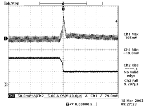
100% to 50% load 3.3 Vdc Input 1.8 Vdc Output
