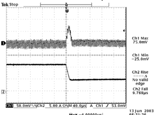
100% to 50% load 3.3 Vdc Input 1.5 Vdc Output
