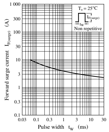
I_{F(\text{surge})} - t_w
