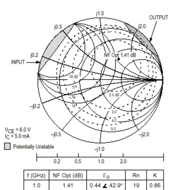
Fig. 22 Constant Gain & Noise Figure Coutours
