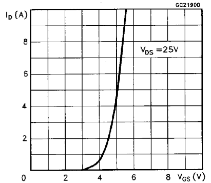
Transfer Characteristics
