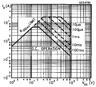
Safe Operating Areas For TO-220
