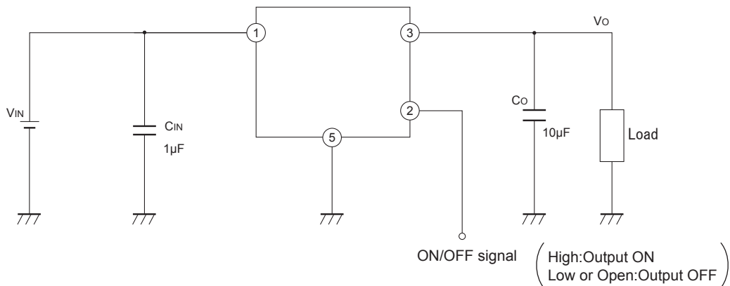
Fig.1 Typical Application
