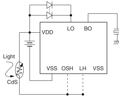
Circuit 3
