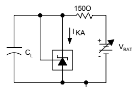
TEST CIRCUIT FOR CURVE A
