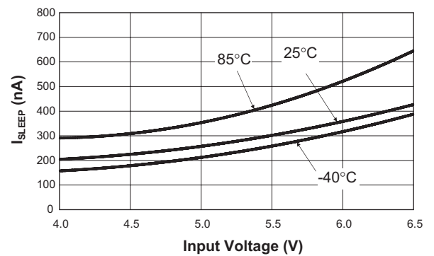
Sleep Mode Current vs. Input Voltage ( R_{SET} = 8.06k\Omega )
