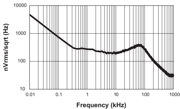
LDO Output Noise
