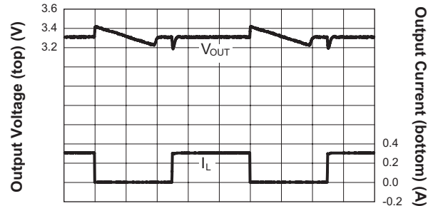
Load Transient Response (1mA to 300mA; V_{IN} = 5.0\text{V} ; V_{OUT} = 3.3\text{V} )
