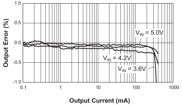
DC Regulation ( V_{OUT} = 3.3V ; L = 5.6\mu H )
