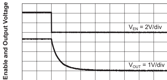
Turn-Off Response Time ( V_{IN} = 4.2\text{V} ; I_{OUT} = 300\text{mA} )
