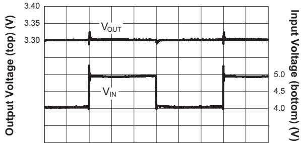
Line Transient Response ( I_{OUT} = 300\text{mA} )
