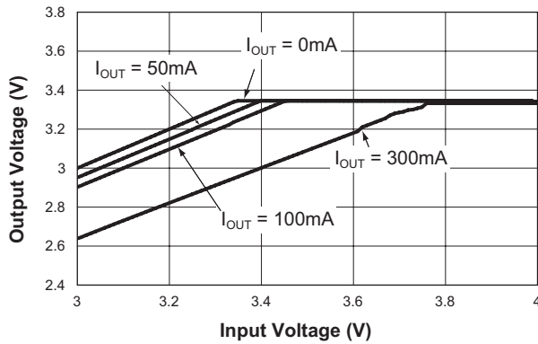
Dropout Characteristics
