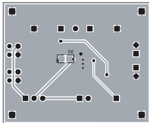
Figure 7: AAT2552 Evaluation Board Bottom Side Layout.
