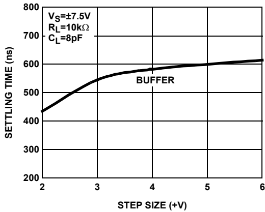
FIGURE 9. SETTling TIME vs STEP SIZE
