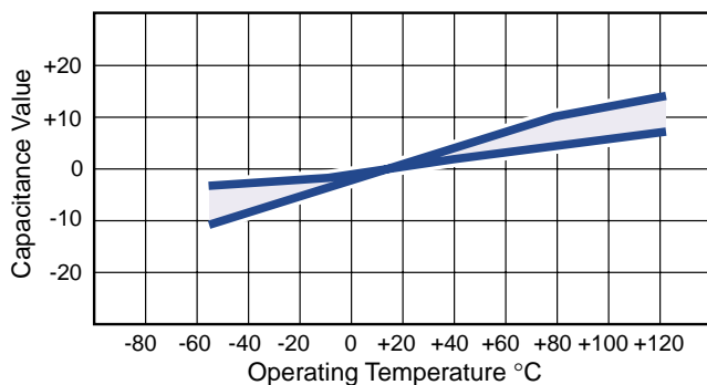
Fig. 1a Typical capacitance with temperature
