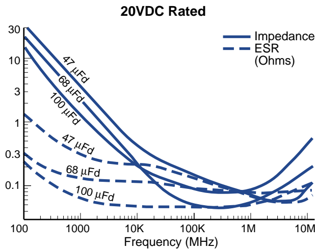
Figure 7b. ESR and Impedance vs. Frequency
