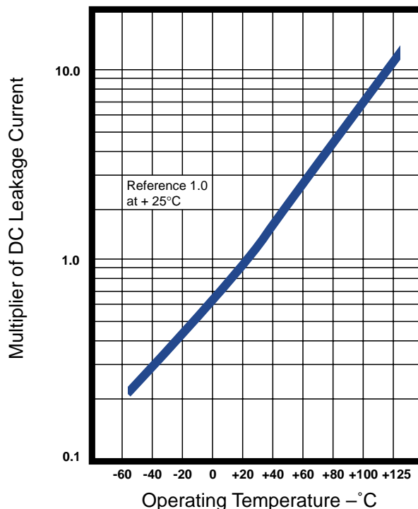
Fig 4 Typical Variation of leakage current with temperature.
