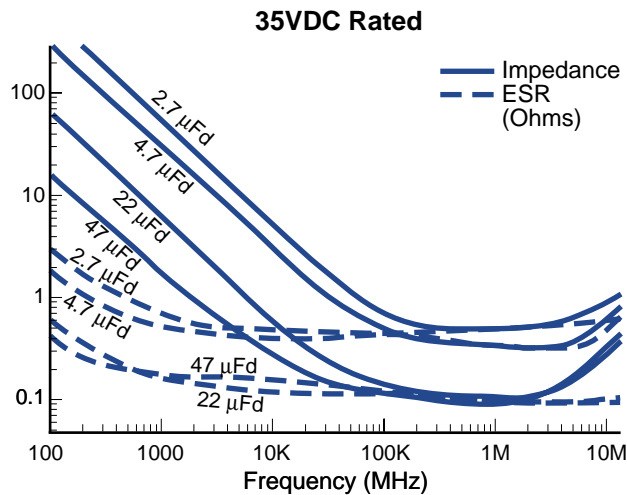
Figure 7c. ESR and Impedance vs. Frequency
