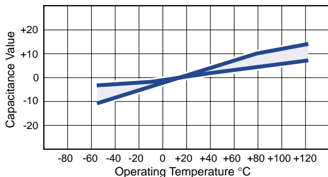
Fig 2 Capacitance Versus Temperature
