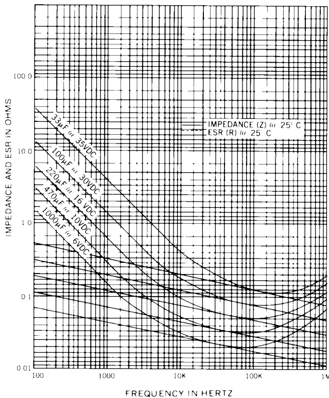
Fig. 6 Typical Behavior of Impedance and ESR as a function of frequency @ 25°C
