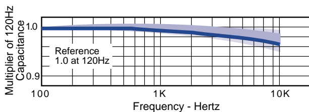
Fig. 1b Typical Variation of capacitance with frequency @ 25° C
