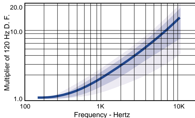
Fig 3 Frequency - Hertz
