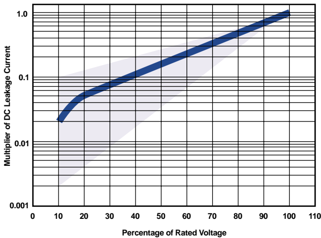
Fig 5 Typical variation of leakage current with voltage
