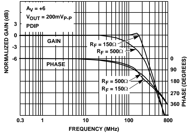
FIGURE 29. FREQUENCY RESPONSE
