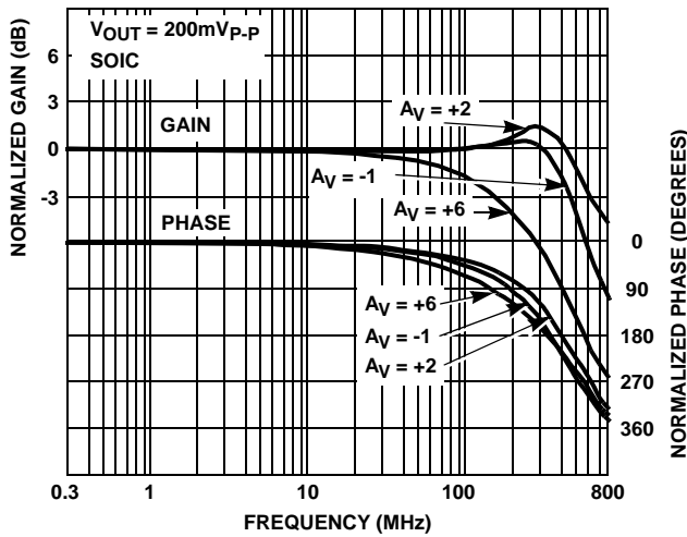
FIGURE 12. FREQUENCY RESPONSE
