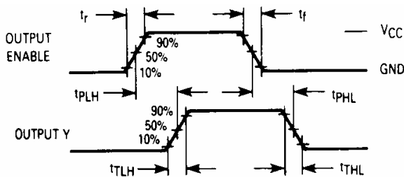
Figure 3. Switching Waveforms
