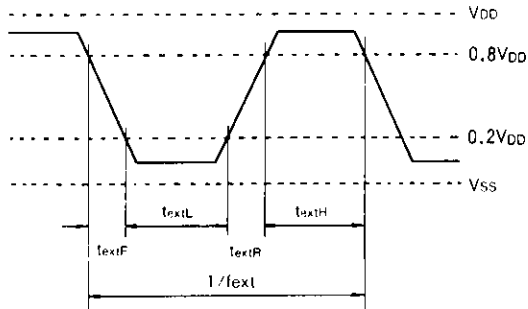
Figure 1 External Clock Input Waveform
