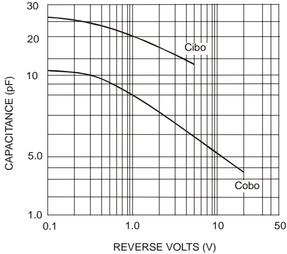
Fig. 3 Typical Capacitance
