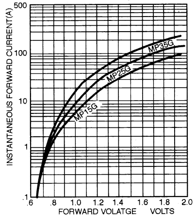
FIG. 4 - TYPICAL FORWARD CHARACTERISTICS - PER ELEMENT
