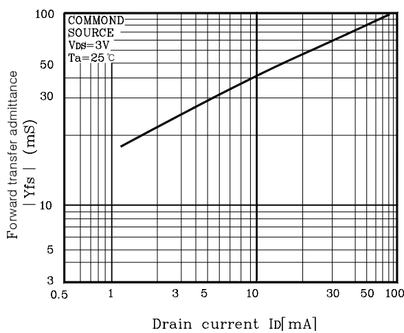
Fig.5 |Yfs| - Id
