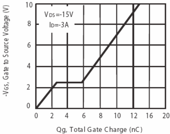
Figure 9. Gate Charge
