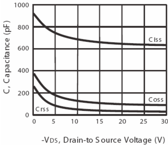
Figure 3. Capacitance
