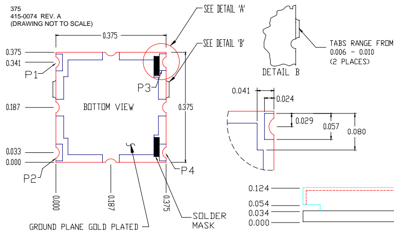
PHYSICAL DIMENSIONS
