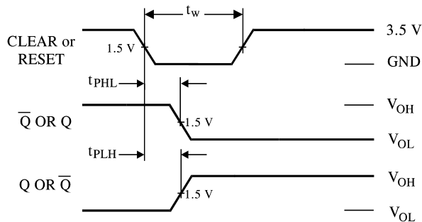
Figure 1. Switching Waveforms
