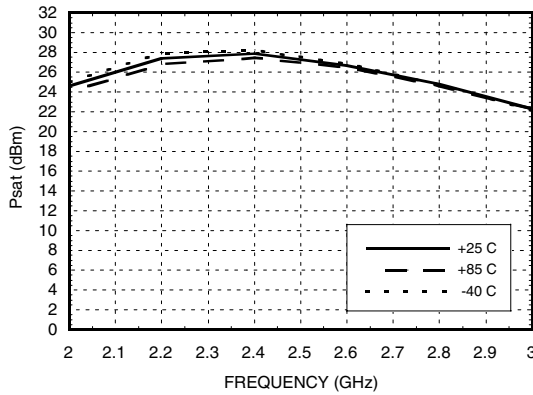
Psat vs. Temperature, Vs= 3.6V
