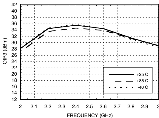
Output IP3 vs. Temperature, Vs= 3.6V
