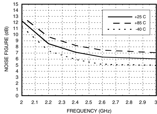
Noise Figure vs. Temperature, V_s = 5.0V
