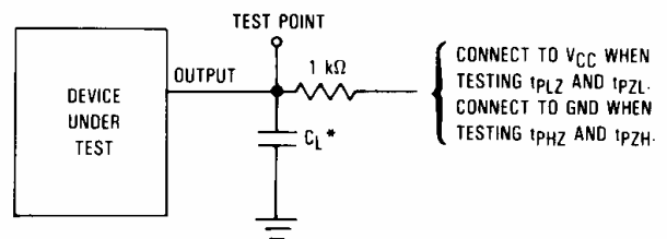
Figure 10. Test Circuit
