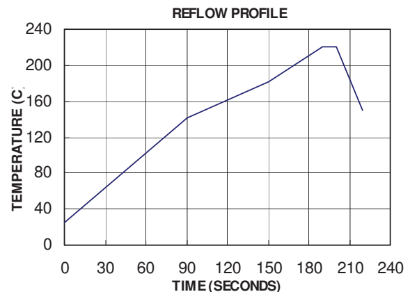
Figure 15 VPOL16A-12-SMT Reflow Profile
