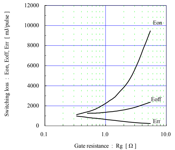
Switching loss vs. Gate resistance (typ.) V_{cc}=900V, I_c=3600A, V_{GE}=\pm 15V, T_j=125^\circ C
