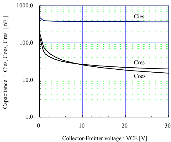
Capacitance vs. Collector-Emitter voltage (typ.) V_{GE}=0V, f=1\text{MHz}, T_j=25^\circ\text{C}
