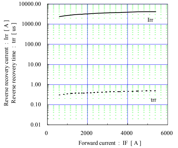
Reverse recovery characteristics (typ.) Vcc=900V, VGE=±15V, Rg=0.1Ω, Tj=125°C
