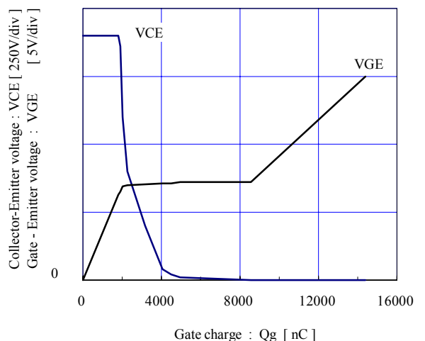
Dynamic Gate charge (typ.) T_j=25^\circ\text{C}
