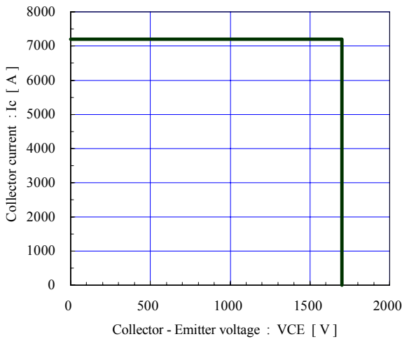
Reverse bias safe operating area (max.) \pm V_{GE}=15V, T_j=125^\circ C / \text{chip}
