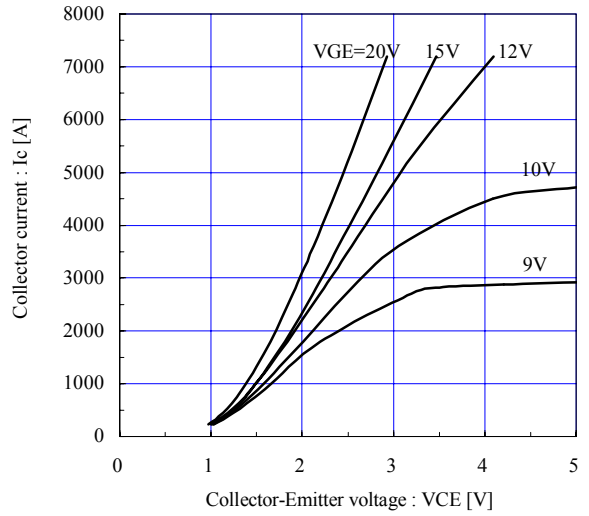
Collector current vs. Collector-Emitter voltage (typ.) T_j=125^\circ\text{C}, \text{sense terminal}
