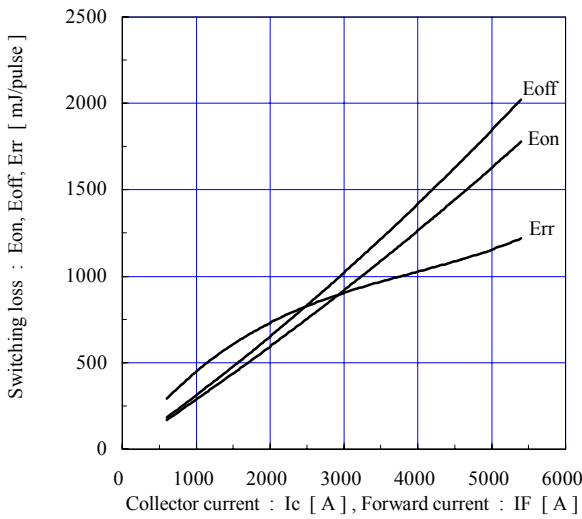
Switching loss vs. Collector current (typ.) V_{cc}=900V, V_{GE}=\pm 15V, R_{gon}=0.1\Omega, R_{goff}=0.2\Omega, T_j=125^\circ C
