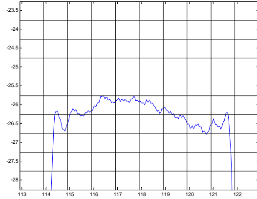
Phase Linearity( f_0 \pm 3.5 MHz)
