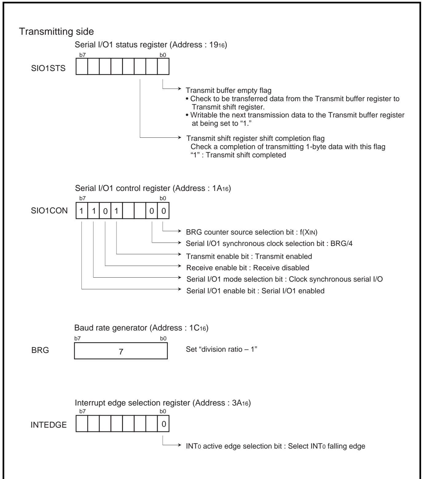
Fig. 2.3.19 Setting of related registers at a transmitting side [Communication using a clock synchronous serial I/O]
