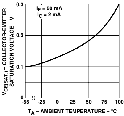
Figure 7. Collector-emitter saturation voltage vs. temperature.
