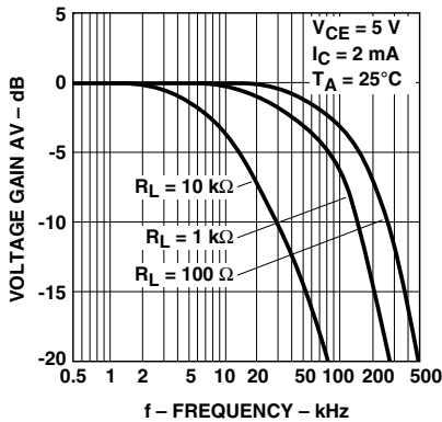
Figure 10. Frequency response.
