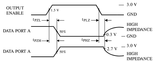
Figure 5. Switching Waveforms
