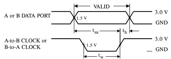
Figure 7. Switching Waveforms
