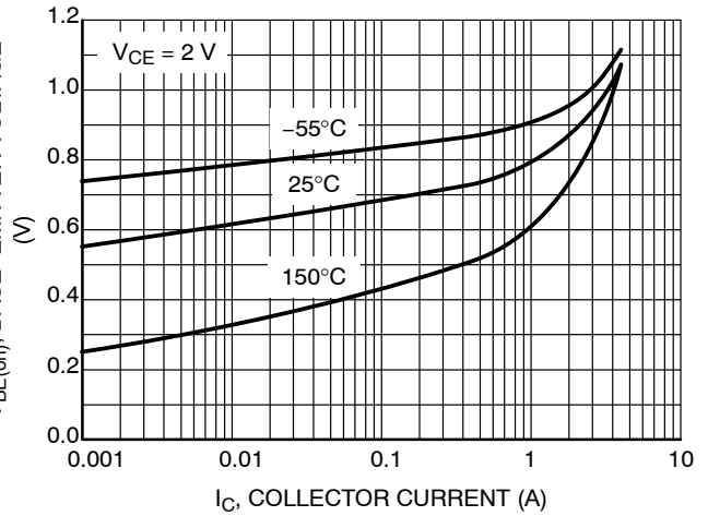
Figure 8. Base-Emitter Voltage
