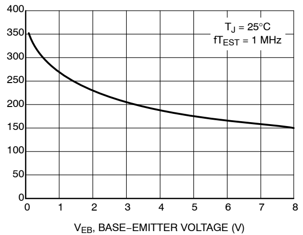
Figure 10. Input Capacitance
