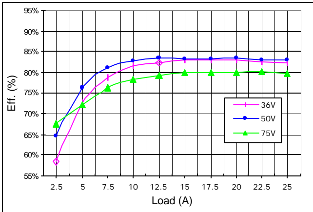
Figure 14. Efficiency at nominal output voltage vs. output current for various Input voltage. The unit mounted on the 0.06" thick PCB with 300LFM air flow (1.5/m) from pin 3 to pin 4 and Ta=25°C
