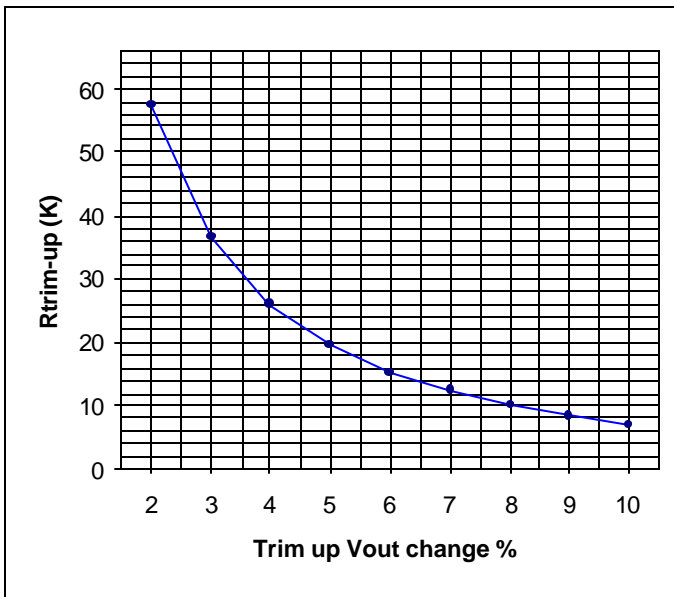
Fig 5. Trim Up Resistance for reference chart
