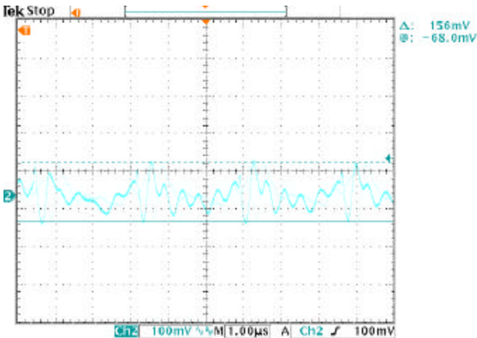
Figure 21. Output voltage Ripple & Noise at Vin=48v, Iout=0A, with 10uF tantalum cap. and 1uf ceramic cap. output capacitance load.
