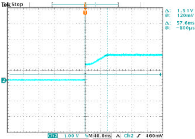
Figure 17. Output voltage over shoot and rise time at Vin=48v, Iout = 0A; with 100uF output capacitance load, and On/Off pin enabled to turn on the unit.
