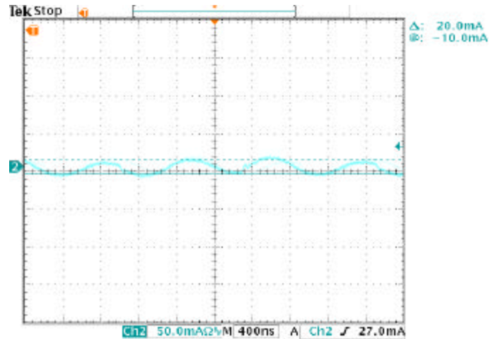
Figure 27. Input reflected ripple current \dot{I}_s waveform With 10uH input inductor. At V_{in}=48v , I_{out}=25A , 50ma/Div ( current probe with 50mv/div)
