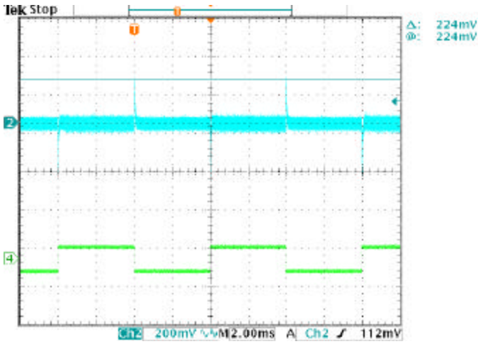
Figure 15. Output voltage dynamic response at Vin=48v Iout= 12~20A, 2.5A/us dynamic load. waveform 2 is dynamic response via dynamic load. waveform 4 is load current (2.5A/us); with 10uF output capacitance load.
