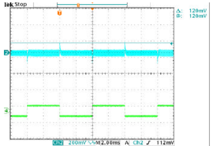
Figure 16. Output voltage dynamic response at Vin=48v Iout= 12~20A, 2.5A/us dynamic load. waveform 2 is dynamic response via dynamic load. waveform 4 is load current (2.5A/us); with 2200uF output capacitance load.
