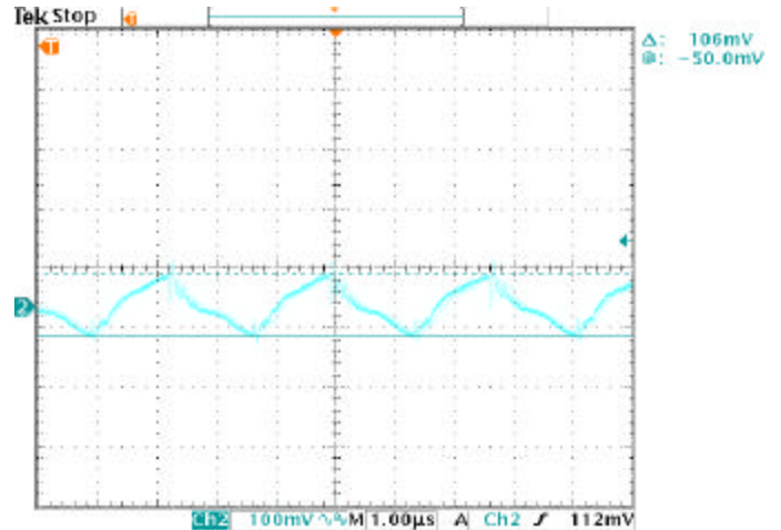
Figure 20. Output waveform under short circuit protection condition. Under 10mΩ short circuit during restart at 48Vin.
