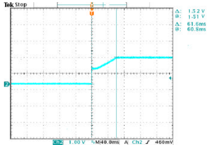
Figure 18. Output voltage over shoot and rise time at Vin=48v, Iout=20A; with 100uF output capacitance load, and On/Off enabled to turn on the unit.
