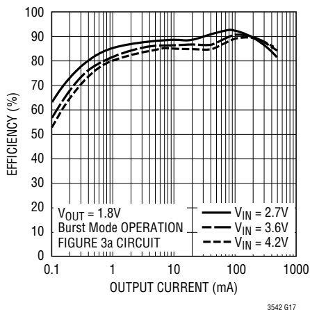
Figure 3c. Efficiency Curve
