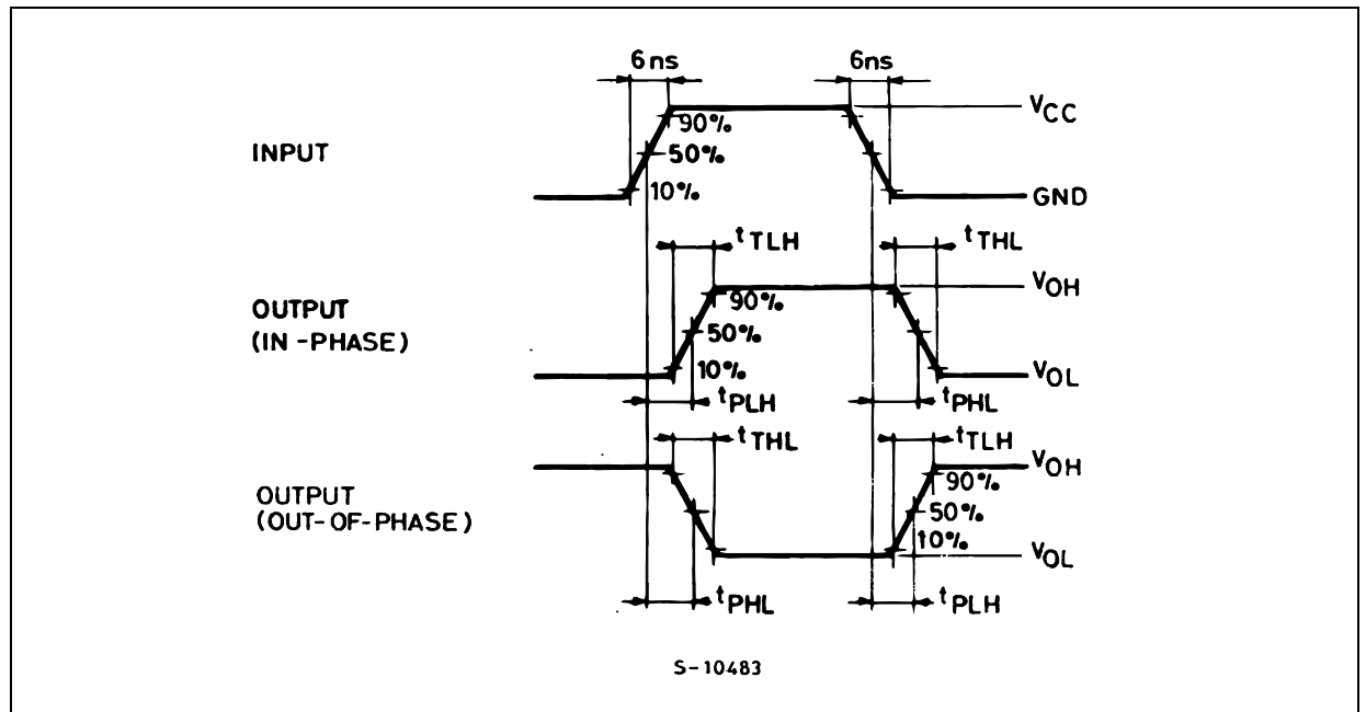
Figure 5: Waveform - Propagation Delay Time ( f=1\text{MHz} ; 50% duty cycle)
