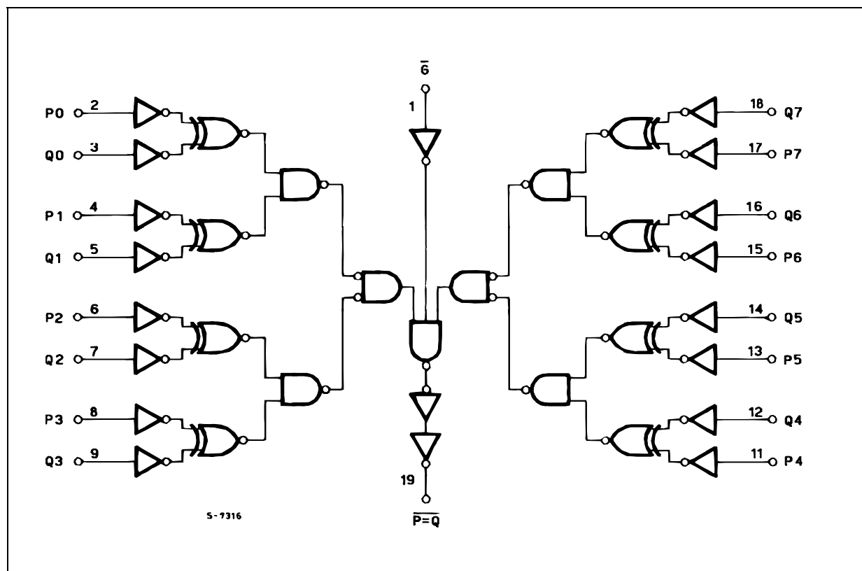
Figure 3: Logic Diagram
