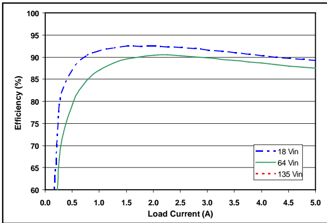
Figure 1: Efficiency at nominal output voltage vs. load current for minimum, nominal, and maximum input voltage at 25°C. (Preliminary)
