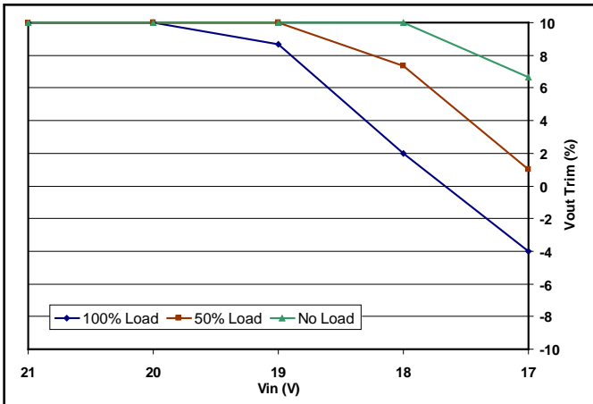
Special Figure 3: Output voltage regulation (trim-up limit) near low-line input for 15 Vout. (Preliminary data)
