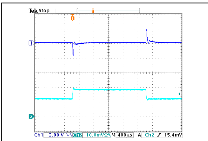
Figure 5: Output voltage response to step-change in load current (50%-75%-50% of I_{out(max)} ; dI/dt = 0.05 \text{ A}/\mu\text{s} ). Load cap: 1 \mu\text{F} ceramic capacitor. Ch 1: V_{out} (2 V/div), Ch 2: I_{out} (2 A/div).
