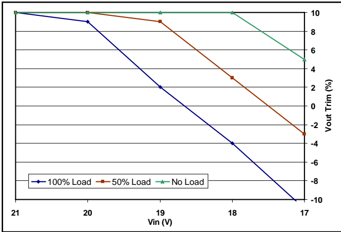
Special Figure 1: Output voltage regulation (trim-up limit) near low-line input for 5 Vout. (Preliminary data)
