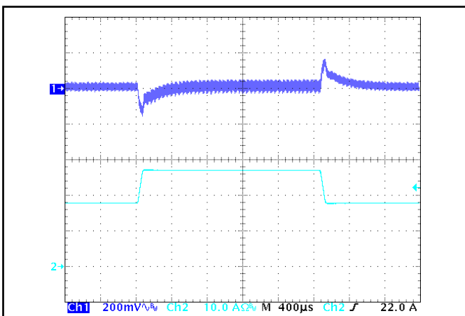
Figure 5: Output voltage response to step-change in load current (50%-75%-50% of I out (max); dI/dt = 0.1 A/μs). Load cap: 1 μF ceramic capacitor. Ch 1: V out (200 mV/div), Ch 2: I out (10 A/div).
