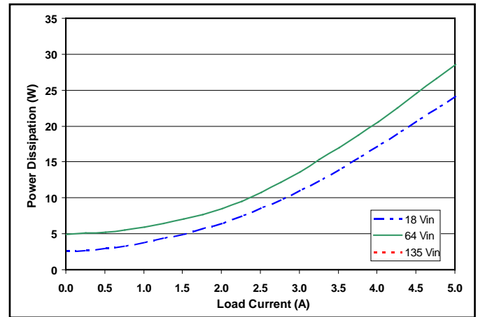
Figure 2: Power dissipation at nominal output voltage vs. load current for minimum, nominal, and maximum input voltage at 25°C. (Preliminary)
