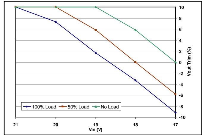
Special Figure 2: Output voltage regulation (trim-up limit) near low-line input for 12 Vout. (Preliminary data)
