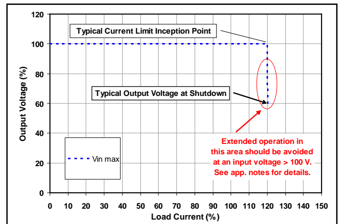
Common Figure 6: Safe operating range limitations.
