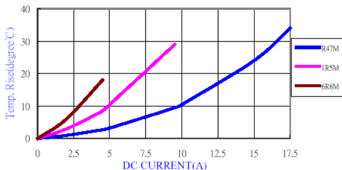
TEMP. RISE VS. DC CURRENT
