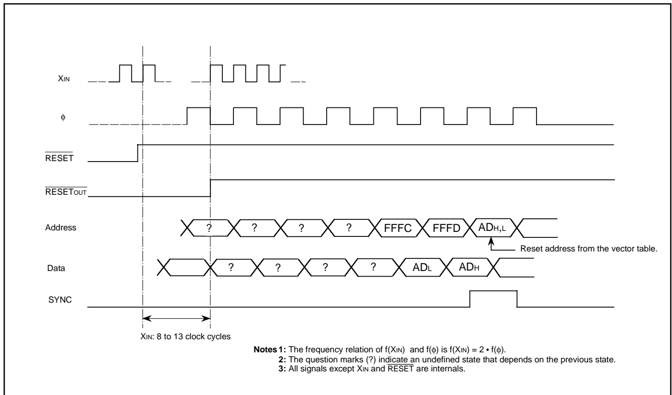
Fig. 40 Reset sequence
