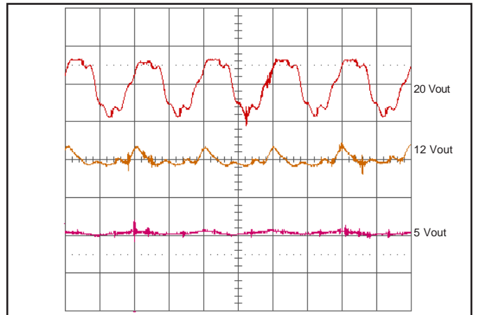
Figure 6: Output Voltage Ripple at 12 V input and rated load current (20 mV/div). Load capacitance: 100 µF electrolytic cap. Bandwidth: 20 MHz. See Figure 4.
