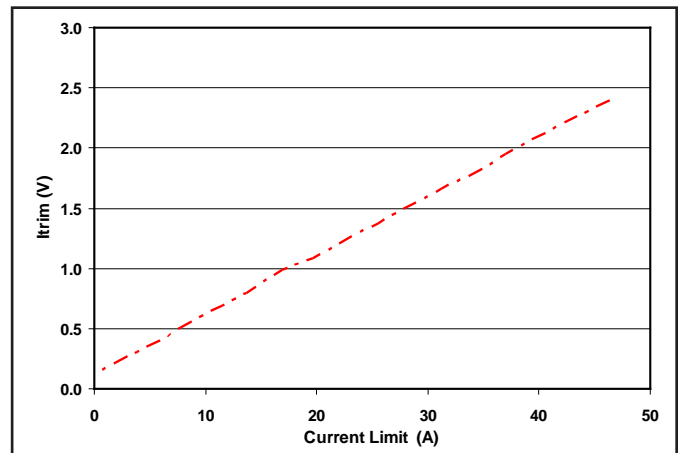
Figure 10: Current limit vs. Itrim pin voltage at 16 V input and 13.8 V output. Load capacitance: 100 \mu F electrolytic cap. C option only.
