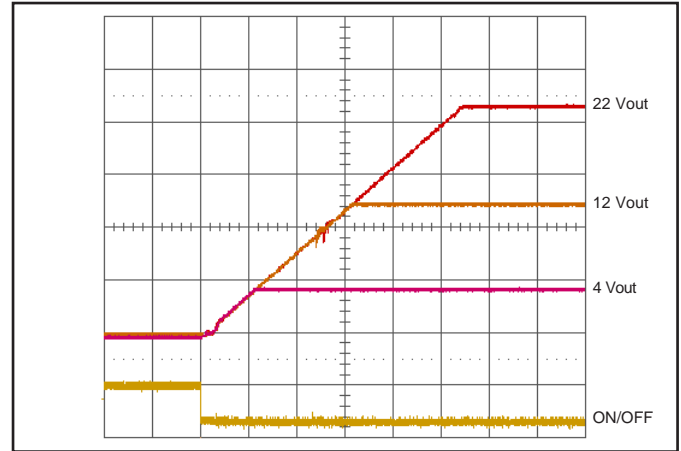
Figure 8: Turn-on transient at 12 V input; full load (20 ms/div). Ch 1: ON/OFF input (5 V/div) Ch 2-4: Vout (5 V/div)
