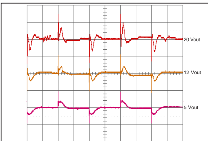
Figure 11: Output voltage response for 12 V input; 5 V, 12 V, 20 V output to step-change in load current (50-75-50% of Iout max; di/dt = 0.1 A/ \mu s). Load cap: 100 \mu F, 100 m \Omega ESR tant, Ch 1-3: Vout (2 V/div);(5 ms/div).
