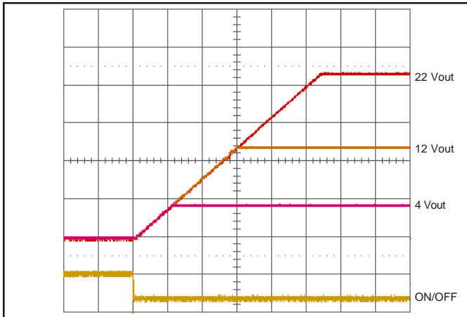
Figure 7: Turn-on transient at 12 V input; zero load (20 ms/div). Ch 1: ON/OFF input (5 V/div) Ch 2-4: Vout (5 V/div)
