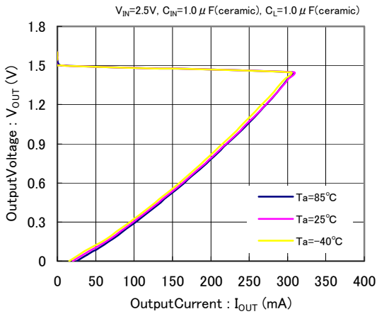
XC6415( V_{OUT}=1.5V )
