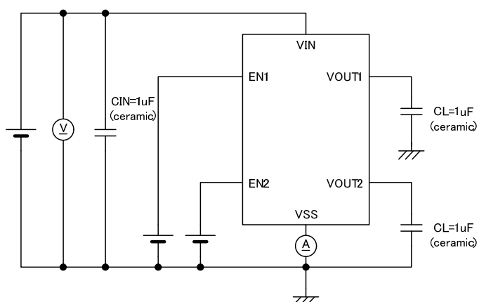
● Circuit ③
