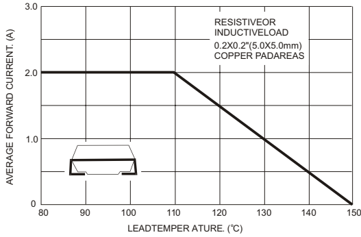
FIG.1-MAXIMUM AVERAGE FORWARD CURRENT DERATING CURVE
