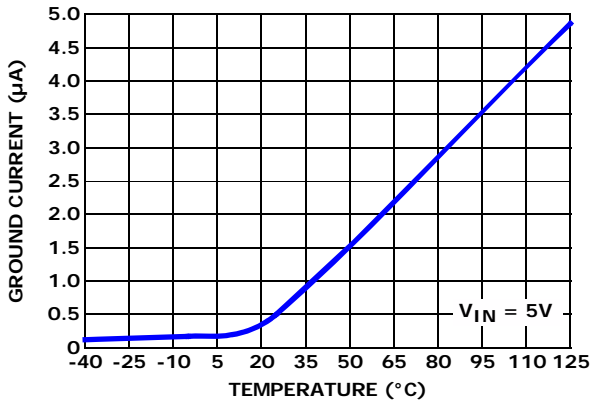
FIGURE 11. SHUTDOWN CURRENT vs TEMPERATURE
