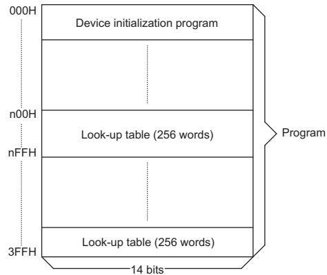
Program Memory
