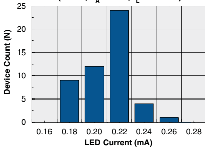
Typical I F for Switch Operation (N=50, T A =25°C, I L =400mA)
