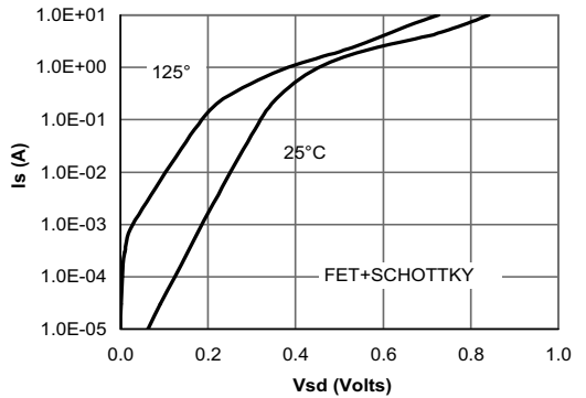
Figure 6: Body-Diode Characteristics (Note 6)
