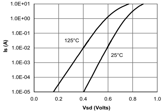
Figure 6: Body-Diode Characteristics
