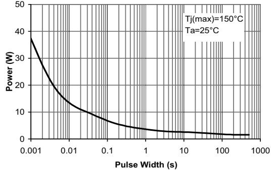
Figure 10: Single Pulse Power Rating Junction-to-Ambient (Note 5)
