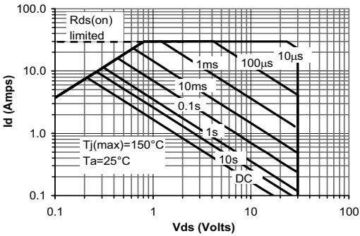
Figure 9: Maximum Forward Biased Safe Operating Area (Note 5)
