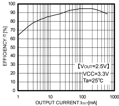
Fig.7 Efficiency
