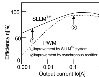
Fig.19 Efficiency
