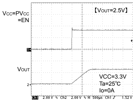
Fig.12 Soft start waveform
