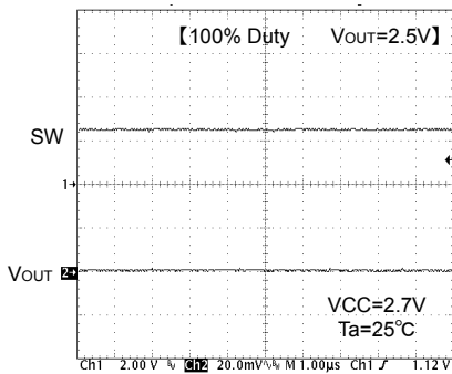
Fig. 15 SW waveform Io=600mA
