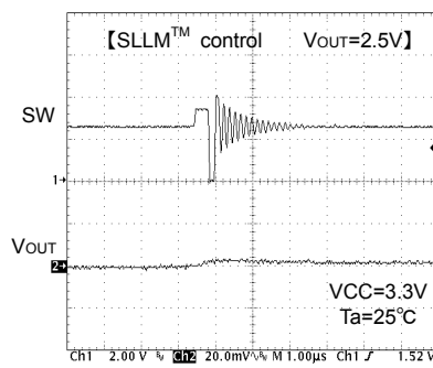
Fig.13 SW waveform Io=10mA
