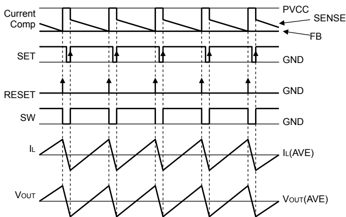
Fig.21 Diagram of current mode PWM control
