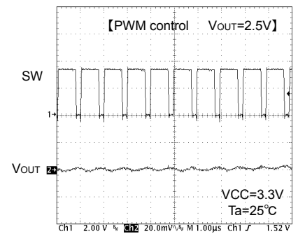
Fig.14 SW waveform Io=500mA
