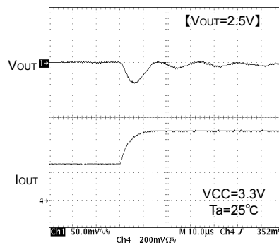
Fig. 16 Transient response Io=250→500mA(10μs)
