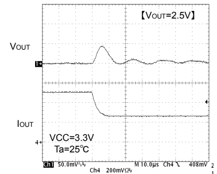
Fig.17 Transient response Io=500→250mA(10μs)
