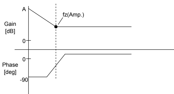
Fig.31 Error amp phase compensation characteristics
