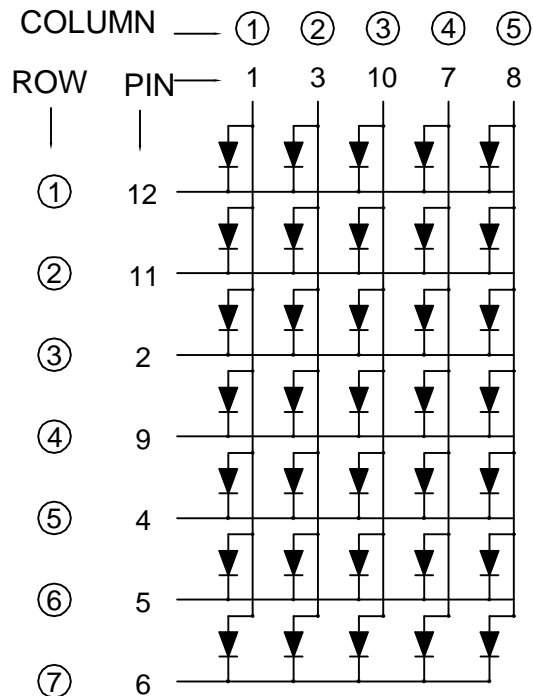
LMD5702ASR-XX-PF
