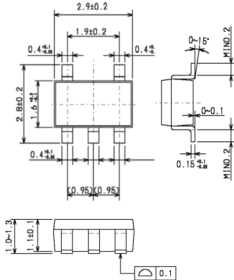
SOT-25 (SOT-23-5)
