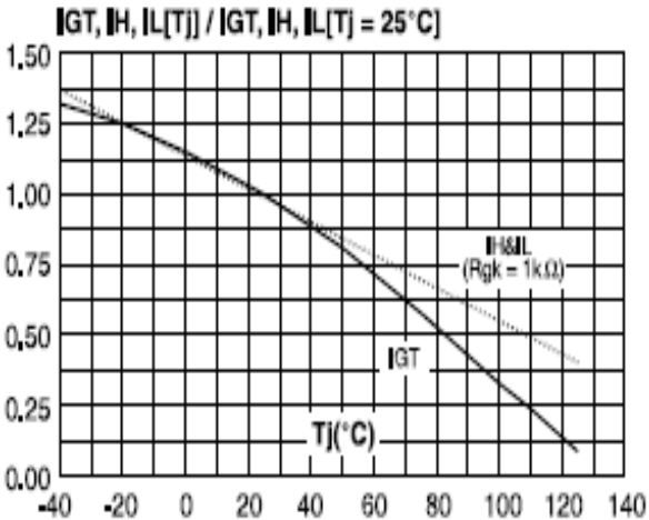
Fig. 3 I_{GT}, I_H, I_L Temperature Characteristics
