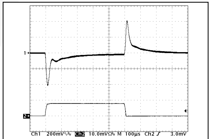
Figure 12: Output voltage response to step-change in load current (0%-50%-0% of Iout(max)). Load cap: 1µF ceramic cap and 10µF, 100 mΩ ESR tantalum cap. Ch 1: Vout (200mV/div). Ch 2: Iout (10A/div).
