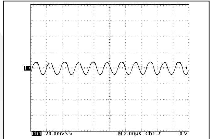
Figure 16: Output voltage ripple, Vout, at nominal input voltage and rated load current (20 mV/div). Load capacitance: 1µF ceramic capacitor and 10µF tantalum capacitor. Bandwidth: 10 MHz. See Figure 14.
