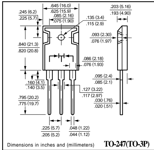
TO-247(TO-3P)
