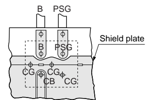
(2) BOTTOM VIEW
