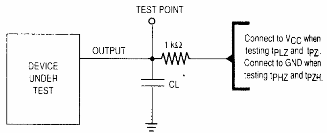
Figure 4. Test Circuit
