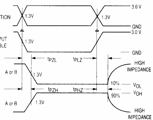
Figure 2. Switching Waveforms
